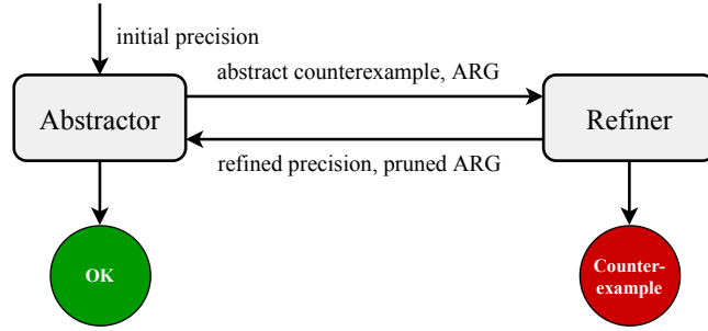
Figure 2.6: The CEGAR-loop.
